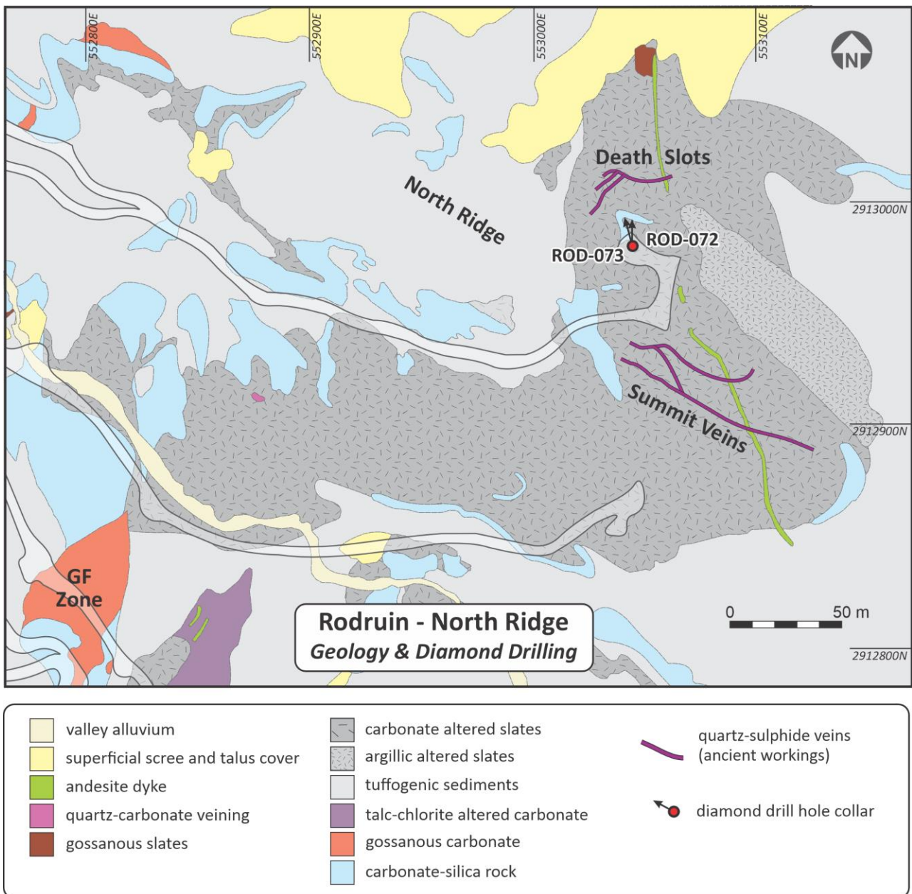
Figure 2: Geological plan of the North Ridge, showing the location of holes ROD-072 and ROD-073
